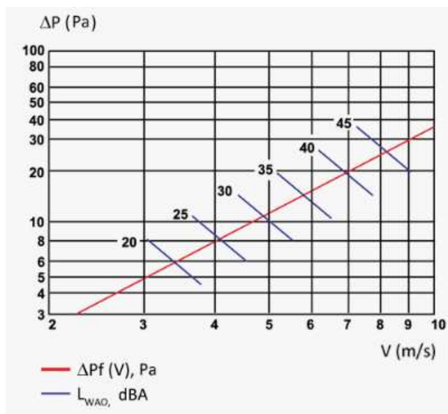
Diagram of pressure losses and sound capacity:
